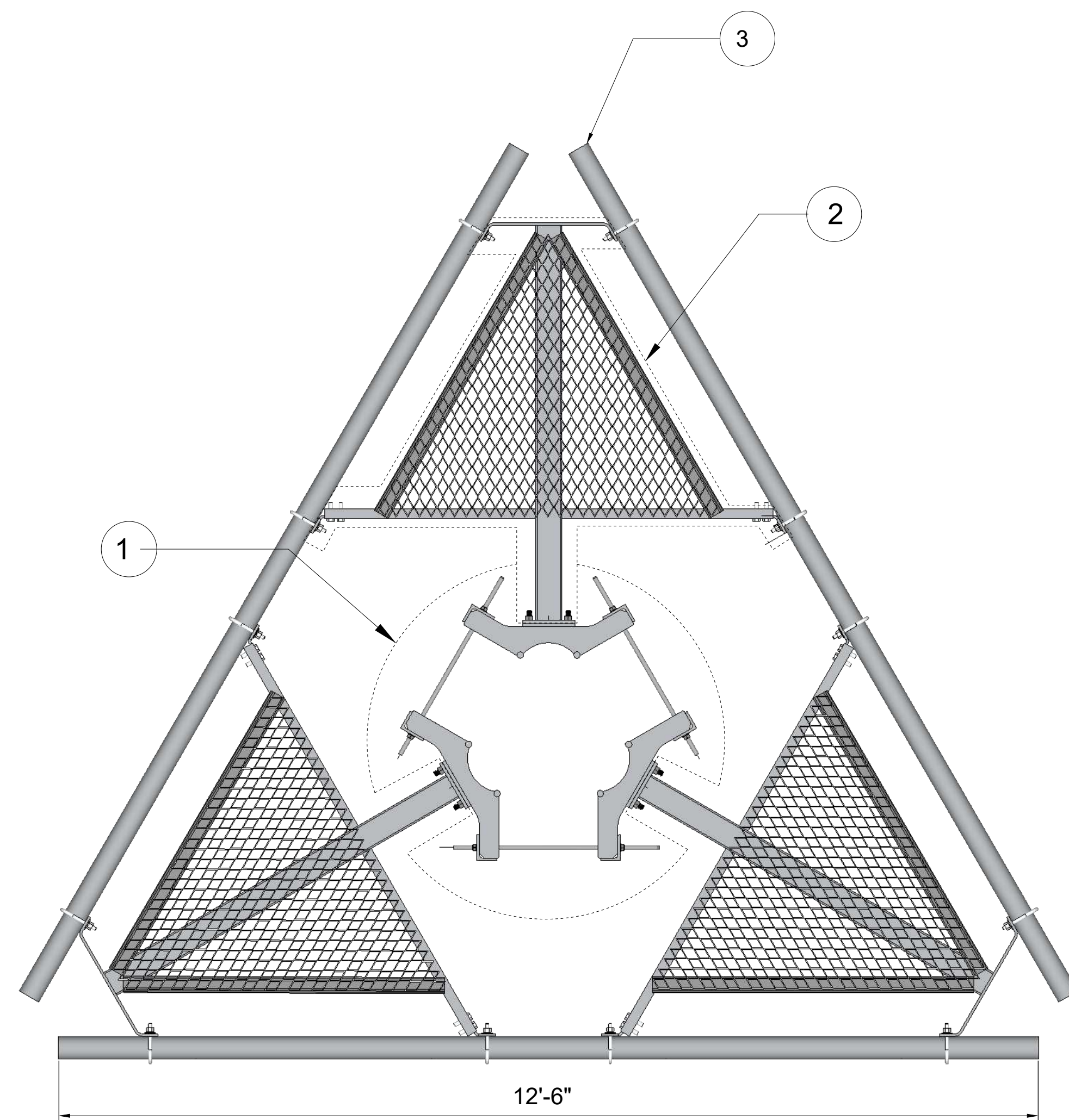
VC-MPT126 - TOP VIEW
