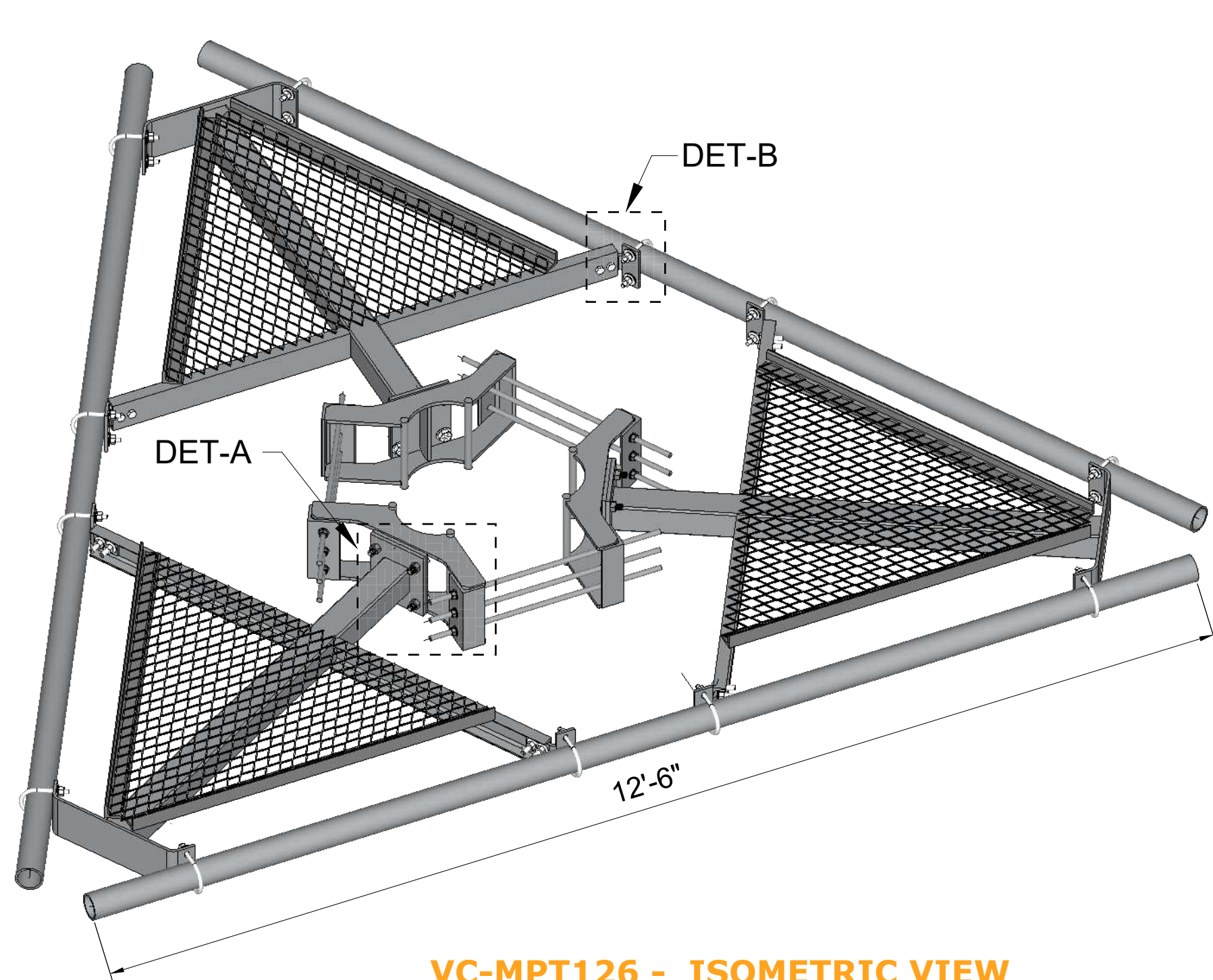
VC-MPT126 - ISOMETRIC VIEW SCALE: 1"=1'-0"(1:12)
