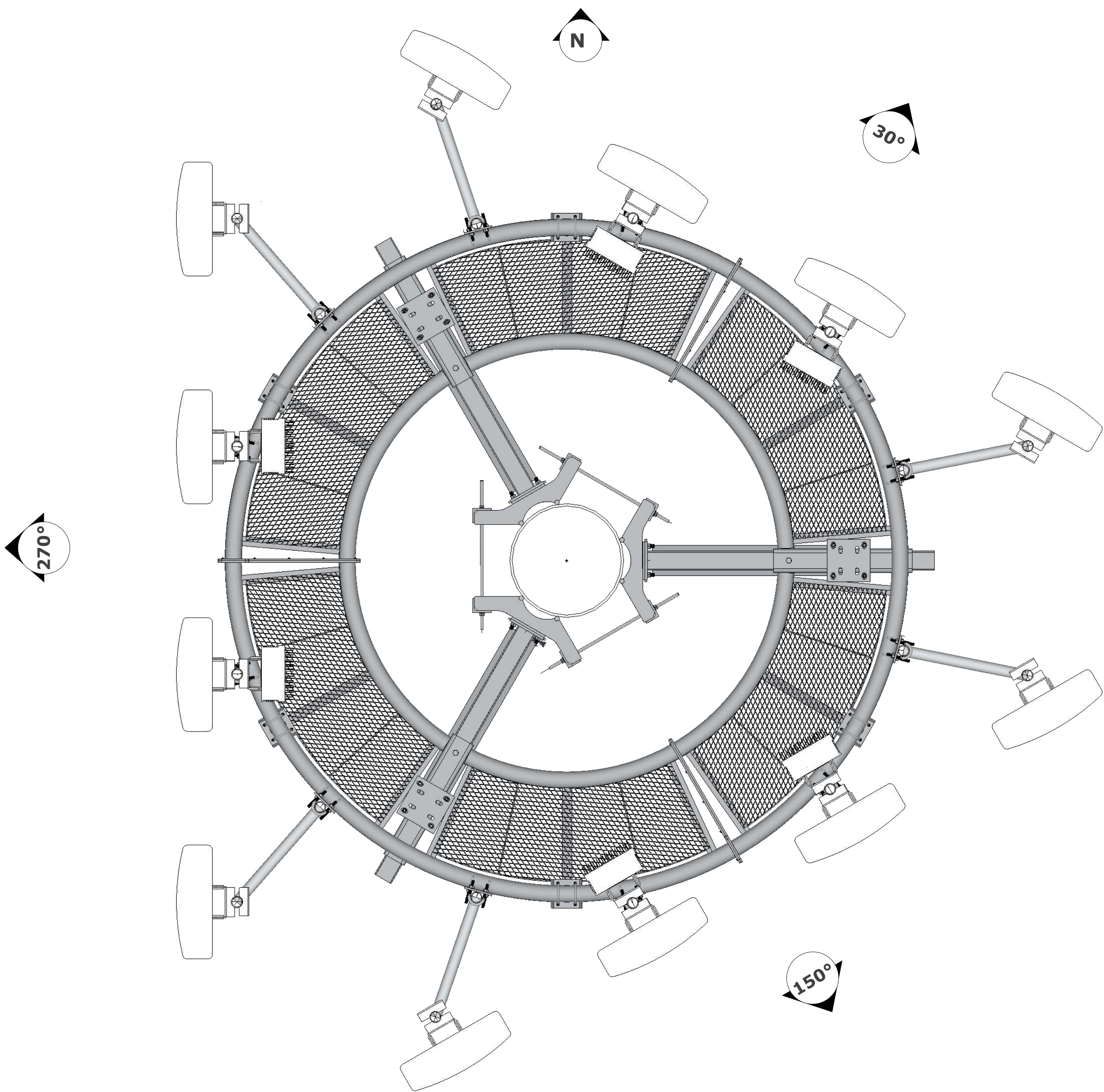
VCMCP12 - APPURTENANCES FINAL ORIENTATION PLAN VIEW
