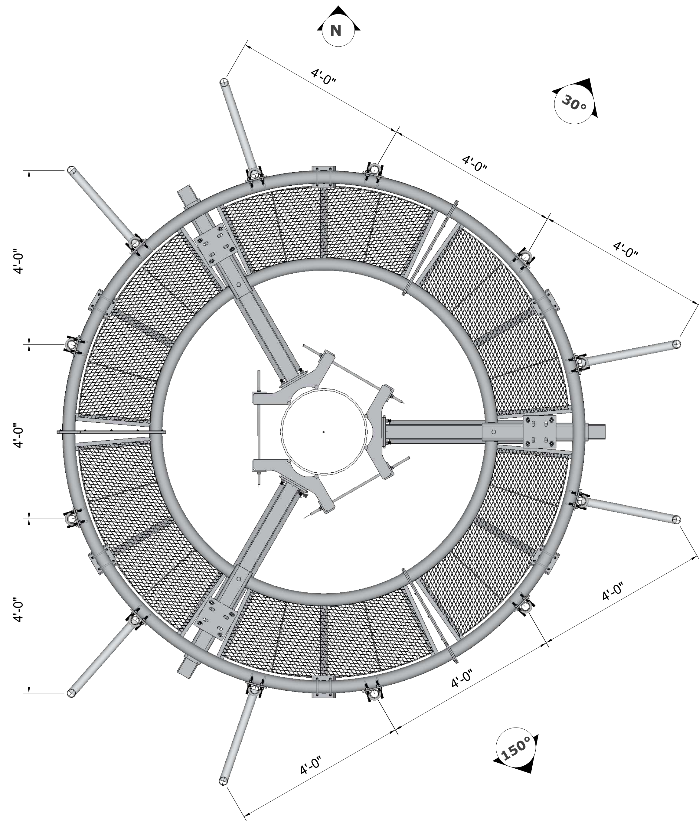
VCMCP12 - PLAN VIEW SCALE: 3/4"=1'-0"(1:16)
