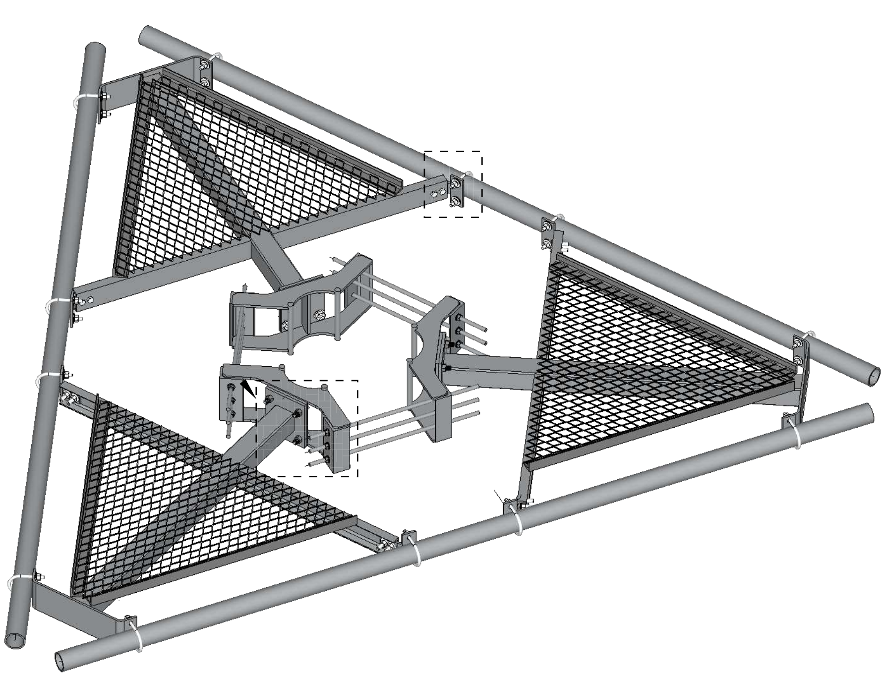
VC-MPT126 - ISOMETRIC VIEW SCALE: 1"=1'-0"(1:12)
